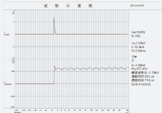
1500V In15A/15.4kA
