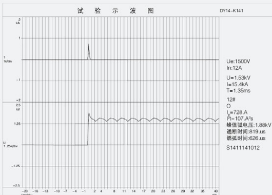
1500V In12A/15.4kA
