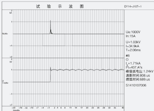
1000V In15A/34.9kA
