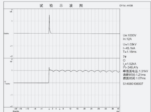
1000V In12A/45.1kA
